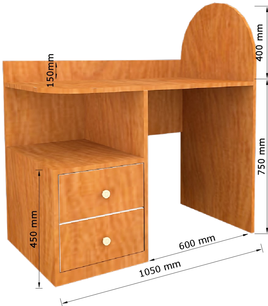
Figure 4: INDICATIVE DESIGN OF HOSTEL STUDY TABLE
