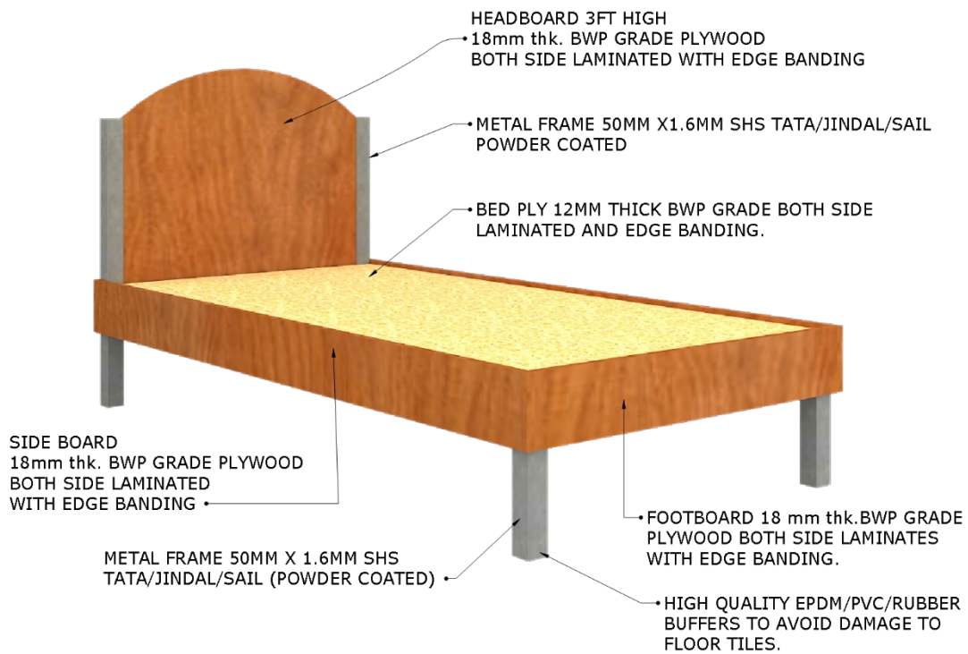
Figure 3: INDICATIVE DESIGN OF HOSTEL BED
