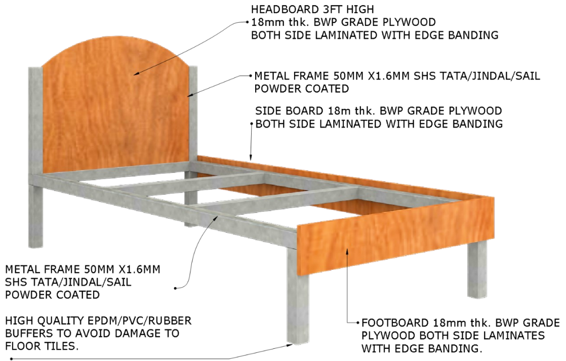
Figure 2: INDICATIVE DESIGN OF HOSTEL BED
