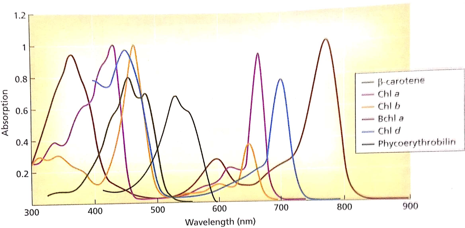
FIGURE 7.7 Absorption spectra of some photosynthetic pigments, including \beta -carotene, chlorophyll a (Chl a ), chlorophyll b (Chl b ), bacteriochlorophyll a (Bchl a ), chloro-
